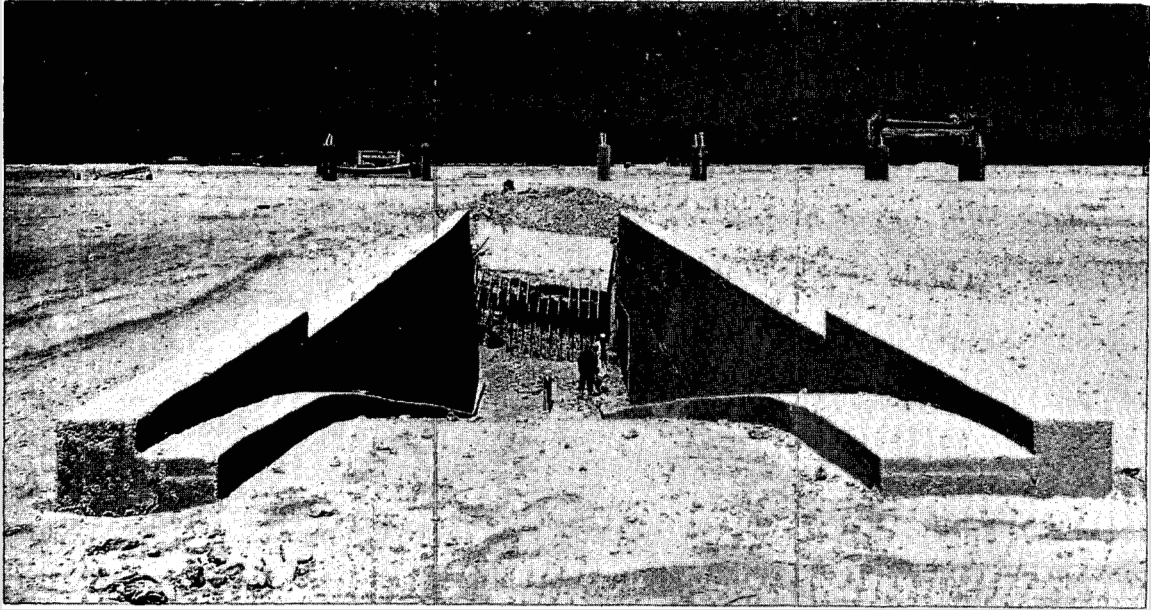
Fig. 1—View of ramp looking toward damaged end wall, postshot.
